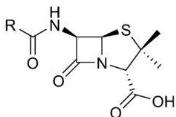
Figure 1. Structure of penicillin core (8)
