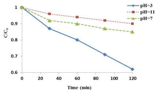
Figure 4. Effect of pH at different time interval on the removal of penicillin G by UV-A process (penicillin G =10 mg/l)
