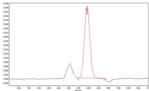
Figure 2. Penicillin G chromatogram
