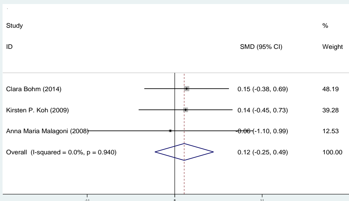
Figure 2. Mean score of the standardized difference of a 6-minute walking test in the control group before and after intervention in all initial studies and the general estimation
