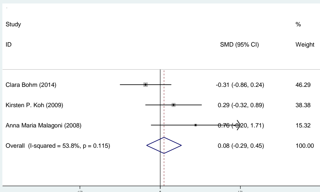
Figure 3. Mean score of the standardized difference of a 6-minute walking test in both experimental and control groups in all initial studies and the general estimation
