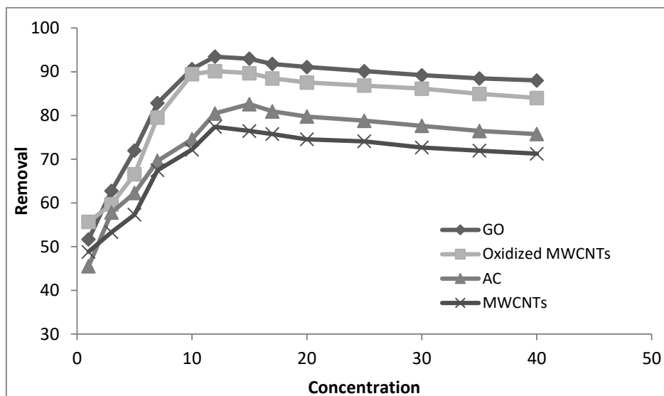
Figure 6. The effect of concentration on the IC by GO, Oxidized MWCNTs, AC and MWCNTs
