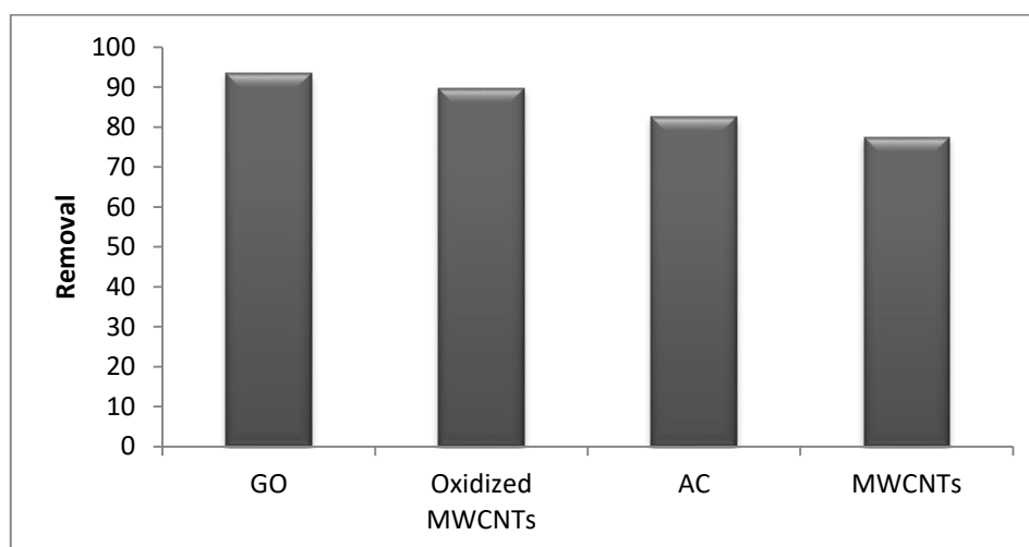
Figure 7. The effect of concentration on removal of IC by GO, Oxidized MWCNTs, AC and MWCNTs
